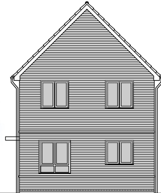
Side Elevation
